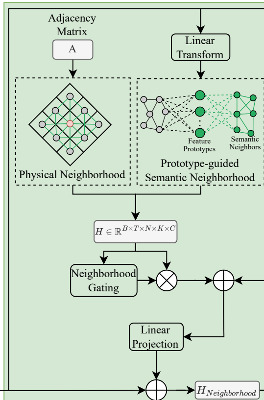
C) Adaptive Neighborhood Aggregator
