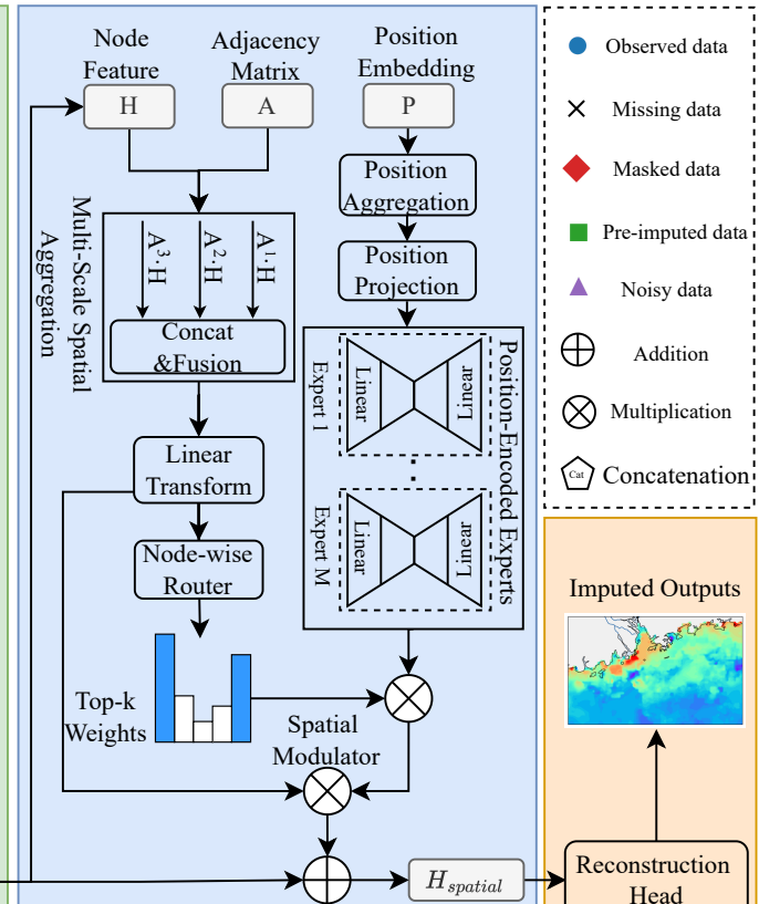
D) Adaptive Heterogeneity Modulator
