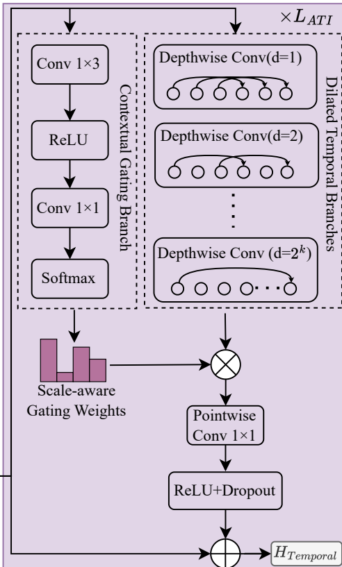
B) Adaptive Temporal Integrator
