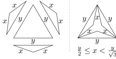
Figure 2: A example of a sextuple of edge lengths, (a, b, c, d, e, f) = (y, y, y, x, x, x) , which satisfies all triangle inequality closure constraints when y \leq 2x , but cannot be the edge lengths of any Euclidean tetrahron when \sqrt{3}x < y .
