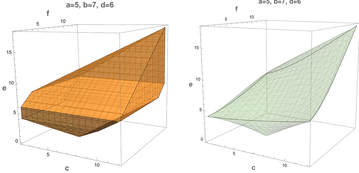
Figure 2: A comparison between the values for (c, e, f) with fixed (a, b, d) = (5, 7, 6) which (left) merely satisfy the triangle inequalities applied to each face the tetrahedron (Eq. (23)) and (right) those which additionally satisfy the Cayley-Menger determinant inequality (Eq. (24)). The figure on the right depicts (a slice of) the moduli space of Euclidean tetrahedra with side lengths (a, b, c, d, e, f) and thus depicts the solution to the tetrahedral Horn problem for 2 \times 2 traceless Hermitian matrices; remark that it is neither a polytope or convex. The figure on the left depicts (a slice of) a polytope, formed by the triangle inequalities (Eq. (23)) which forms a loose outer approximation to the figure on the right.
