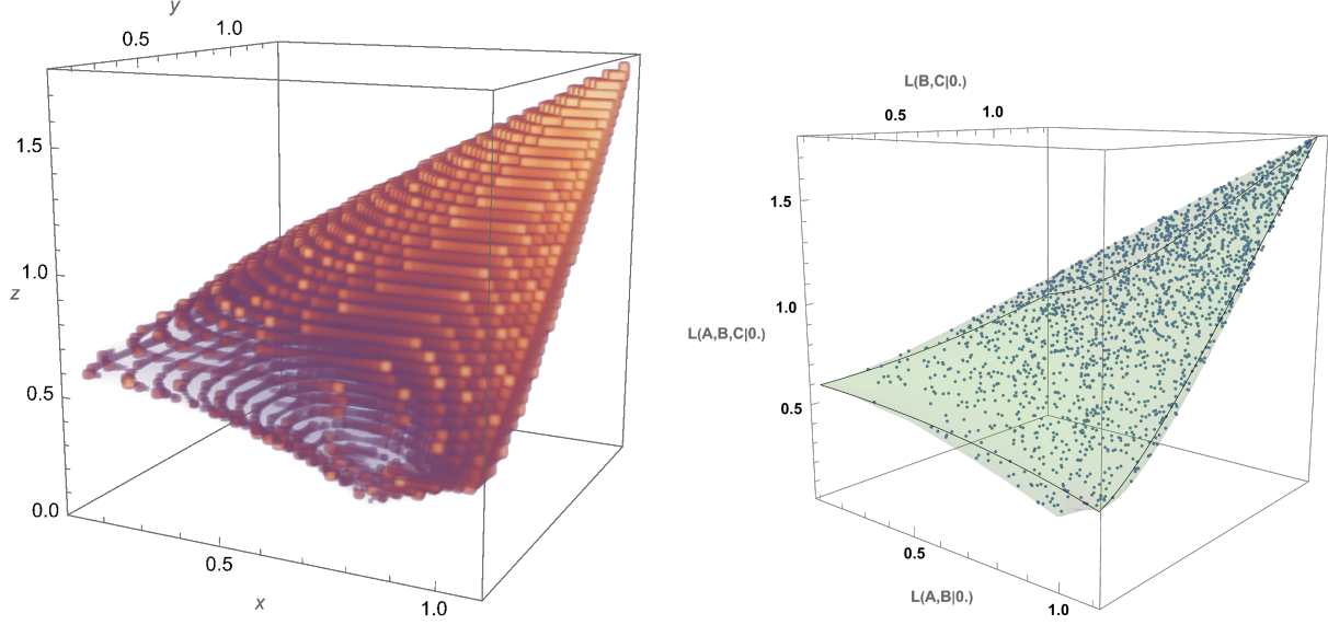
Figure 5: Admissible eigenvalues of partial sums ( A + B , B + C and A + B + C ) of traceless 2 \times 2 matrices (A, B, C) with spectra (\alpha, \beta, \gamma) = (a, b, c) = (0.5, 0.6, 0.7) . Left is a density plot of the analytic formula p(x, y, z|a, b, c) restricted to the admissible region. Right is a numerical sample with admissible region boundary plotted in green.
