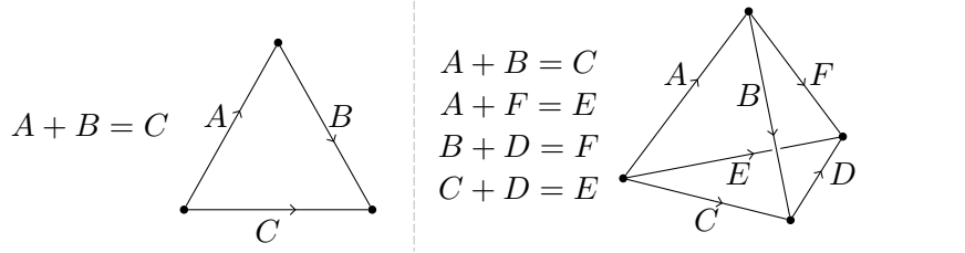
FIGURE 1. (Left) The Horn problem concerns the eigenvalues of three Hermitian matrices, A , B , and C , forming a triangle in \mathcal{H}_n . (Right) The tetrahedral Horn problem concerns the eigenvalues of six Hermitian matrices, A , B , C , D , E , and F , forming a tetrahedron in \mathcal{H}_n . fig:tetrahedron_labelling_scheme
