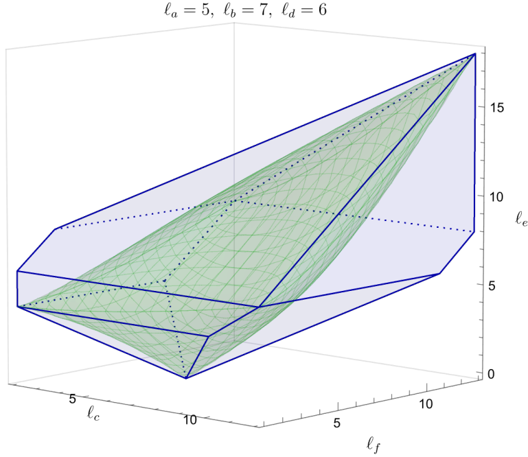
FIGURE 2. The interior green region depicts a slice of the space of side-lengths (\ell_a, \ell_b, \ell_c, \ell_d, \ell_e, \ell_f) of Euclidean tetrahedra where (\ell_a, \ell_b, \ell_d) = (5, 7, 6) and thus depicts a slice of Tetra(2). The exterior blue polytope depicts the values of (\ell_c, \ell_e, \ell_f) which merely satisfy the triangle inequalities, while the interior green region additionally satisfies the Cayley-Menger determinant inequality. fig:tetrahedron_moduli_space_example
