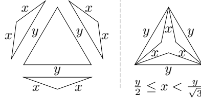
Figure 5: A example of a sextuple of edge lengths, (a, b, c, d, e, f) = (y, y, y, x, x, x) , which satisfies all triangle inequality closure constraints when y \leq 2x , but cannot be the edge lengths of any Euclidean tetrahron when \sqrt{3}x < y .
