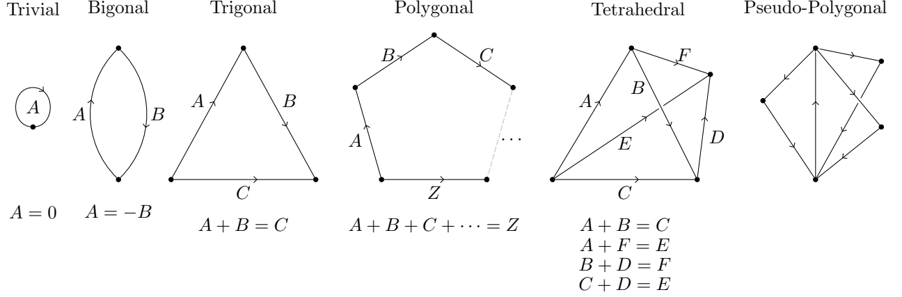
Figure 4: Examples of graphical Horn problems.
