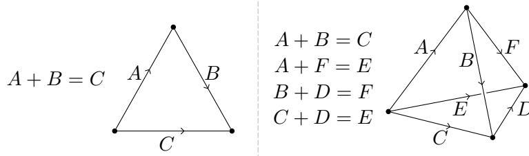
FIGURE 1. (Left) The Horn problem concerns the eigenvalues of three Hermitian matrices, A, B , and C , forming a triangle in \mathcal{H}_n . (Right) The tetrahedral Horn problem concerns the eigenvalues of six Hermitian matrices, A, B, C, D, E , and F , forming a tetrahedron in \mathcal{H}_n .
