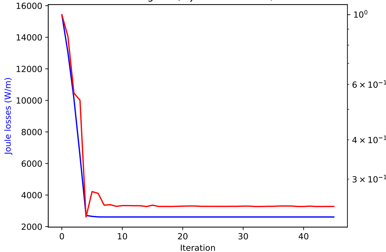
Convergence, P_j = 2.61\text{e}+03 \text{ W/m}
