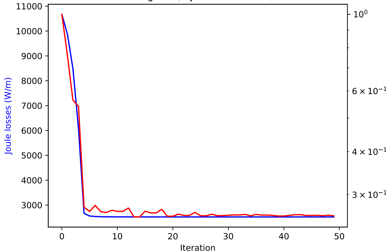
Convergence, P_j = 2.52\text{e}+03 \text{ W/m}
