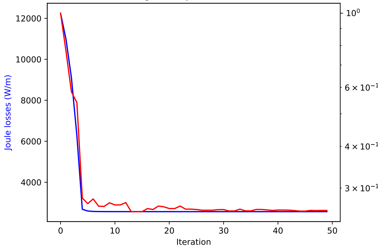
Convergence, P_j = 2.57\text{e}+03 \text{ W/m}
