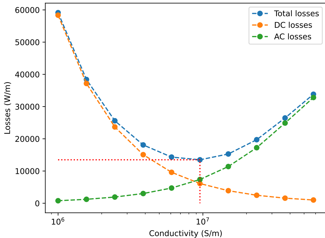
Copper losses (min for \sigma = 9.54\text{e}+06 S/m)
