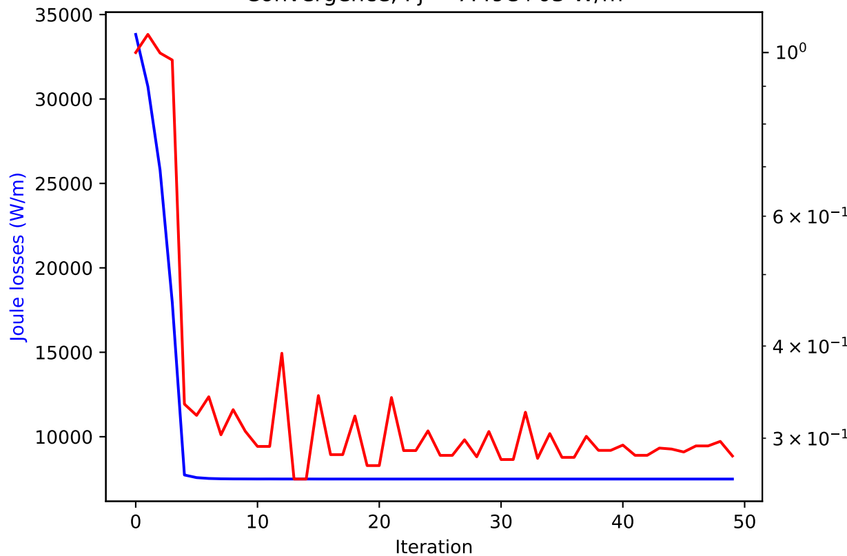
Convergence, P_j = 7.49\text{e}+03 \text{ W/m}
