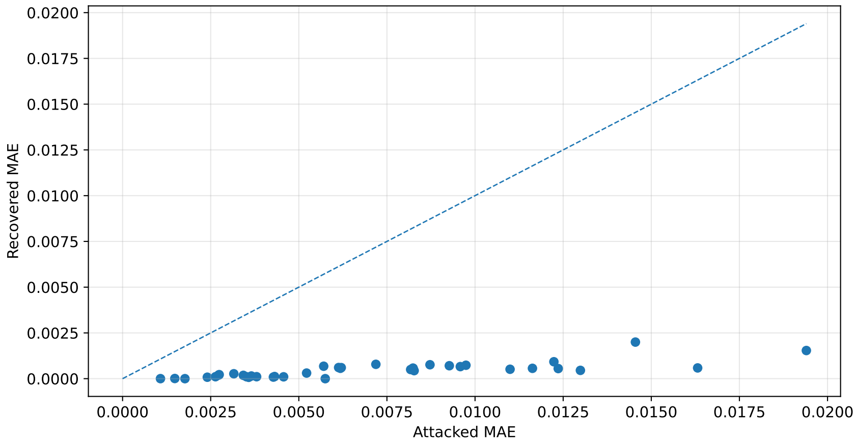
Recovered MAE vs. Attacked MAE
