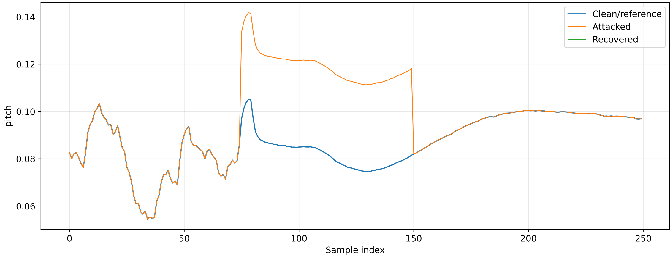
Representative Recovery Result: baseline_01_hover_Pitch_bias_W10_N3_mean1x_detection_OFFICIAL_PHASE5_RECOVERED
