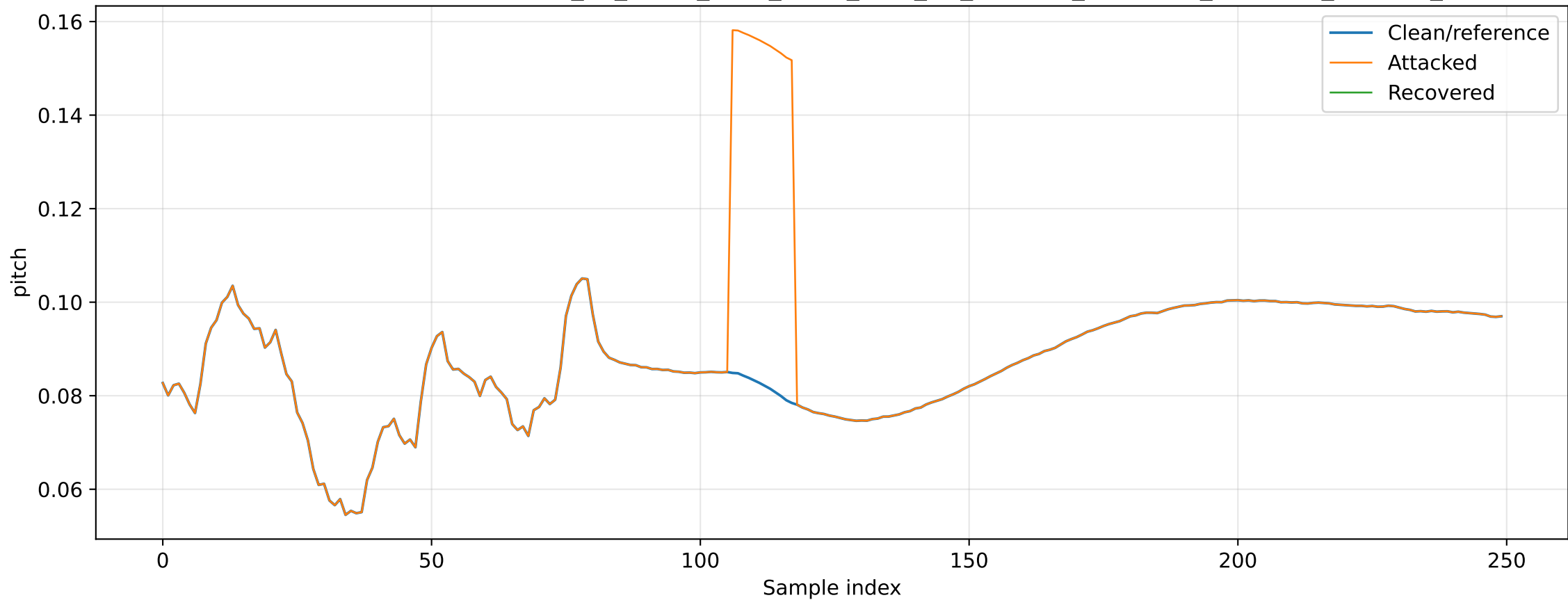
Representative Recovery Result: baseline_01_hover_Pitch_pulse_W10_N3_mean1x_detection_OFFICIAL_PHASE5_RECOVERED
