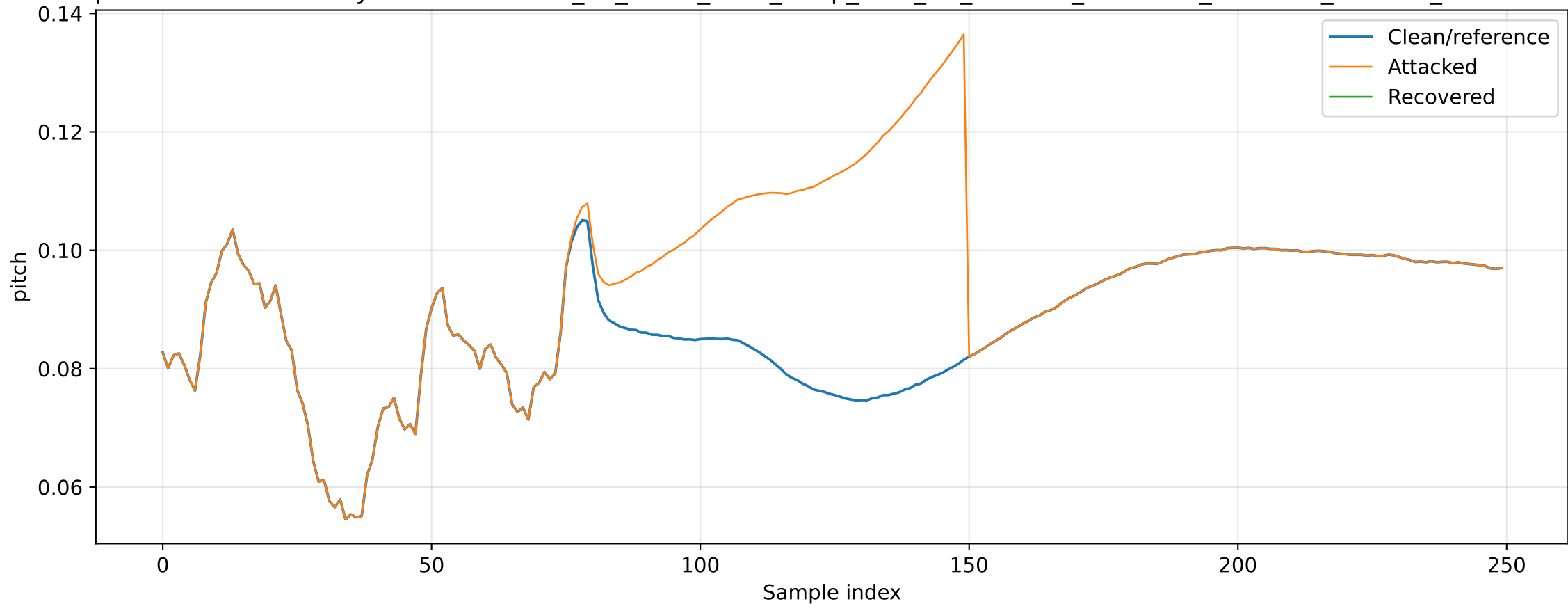
Representative Recovery Result: baseline_01_hover_Pitch_ramp_W10_N3_mean1x_detection_OFFICIAL_PHASE5_RECOVERED
