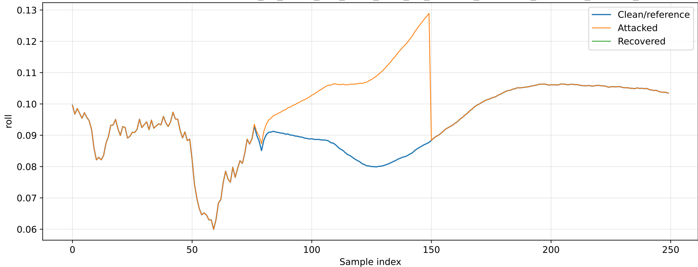
Representative Recovery Result: baseline_01_hover_Roll_ramp_W10_N3_mean1x_detection_OFFICIAL_PHASE5_RECOVERED
