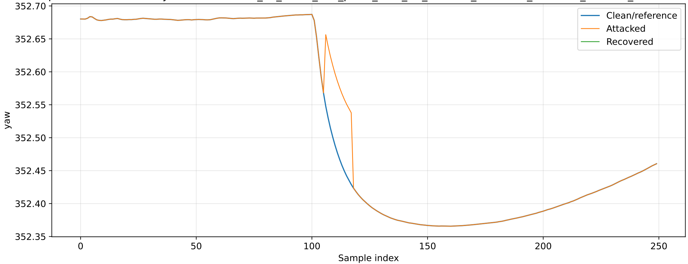
Representative Recovery Result: baseline_01_hover_Yaw_pulse_W10_N3_mean1x_detection_OFFICIAL_PHASE5_RECOVERED
