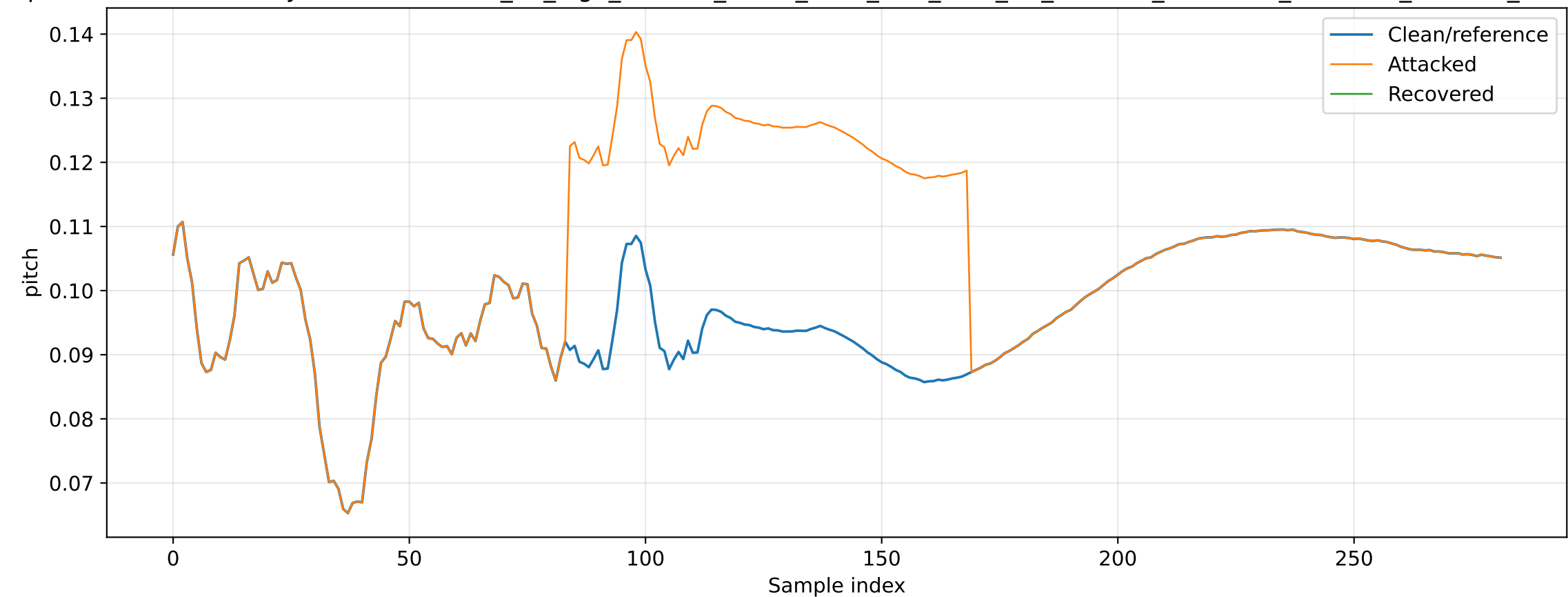
Representative Recovery Result: baseline_02_high_altitude_hover_Pitch_bias_W10_N3_mean1x_detection_OFFICIAL_PHASE5_RECO
