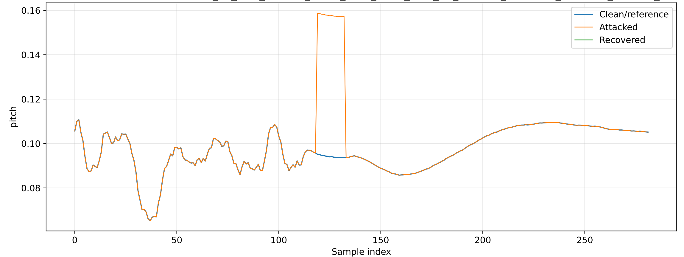
Representative Recovery Result: baseline_02_high_altitude_hover_Pitch_pulse_W10_N3_mean1x_detection_OFFICIAL_PHASE5_REC
