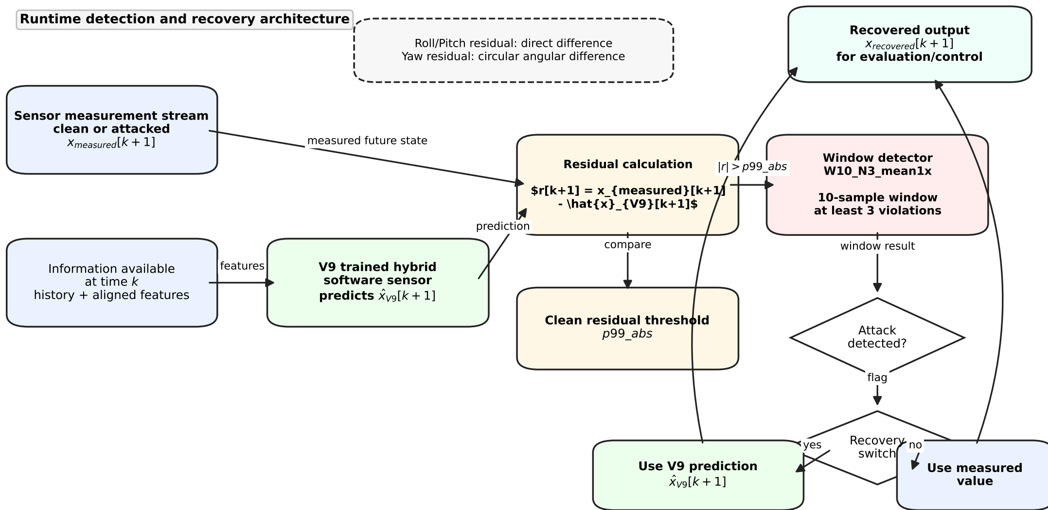
Figure 1. Software-Sensor-Based Attack Detection and Recovery Pipeline
