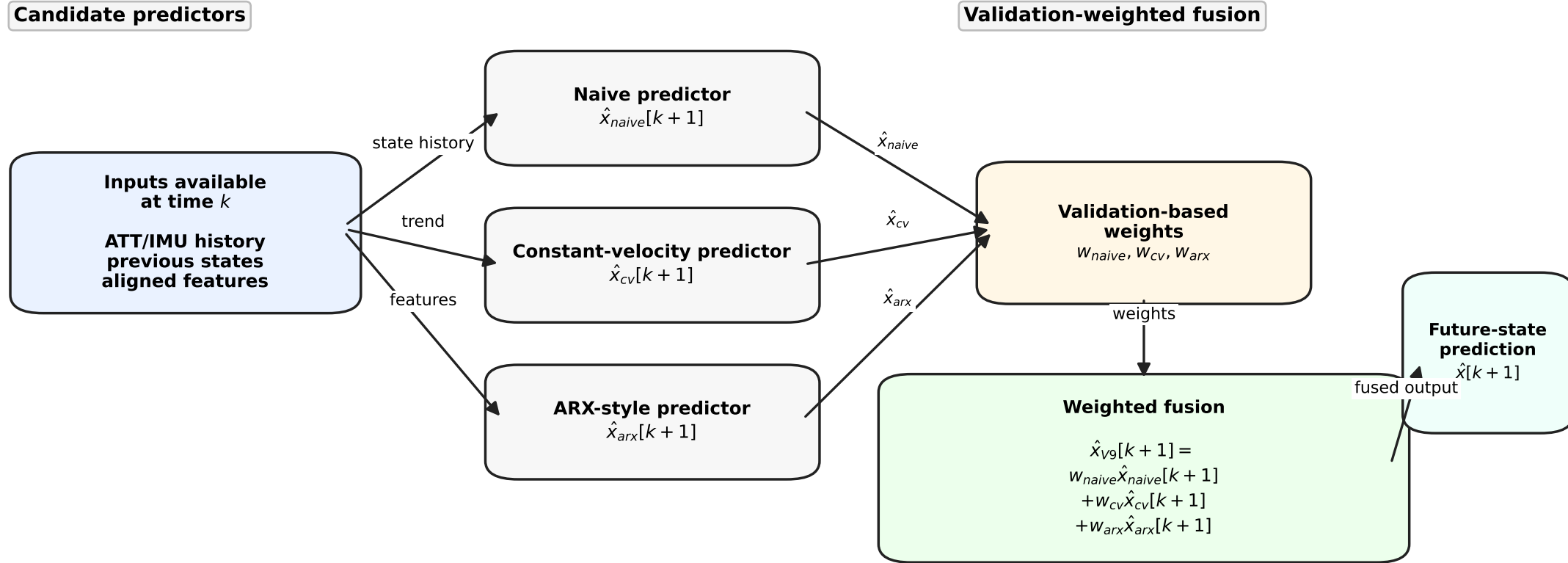
Figure 3. V9 Hybrid Software Sensor Internal Structure
