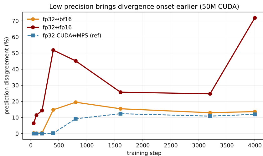
Figure 3: Precision and divergence onset at 50M on CUDA (single seed): fp32↔bf16 and fp32↔fp16, with fp32 CUDA↔MPS for reference. Onset \leq step 50 (fp16) and step 400 (bf16).
