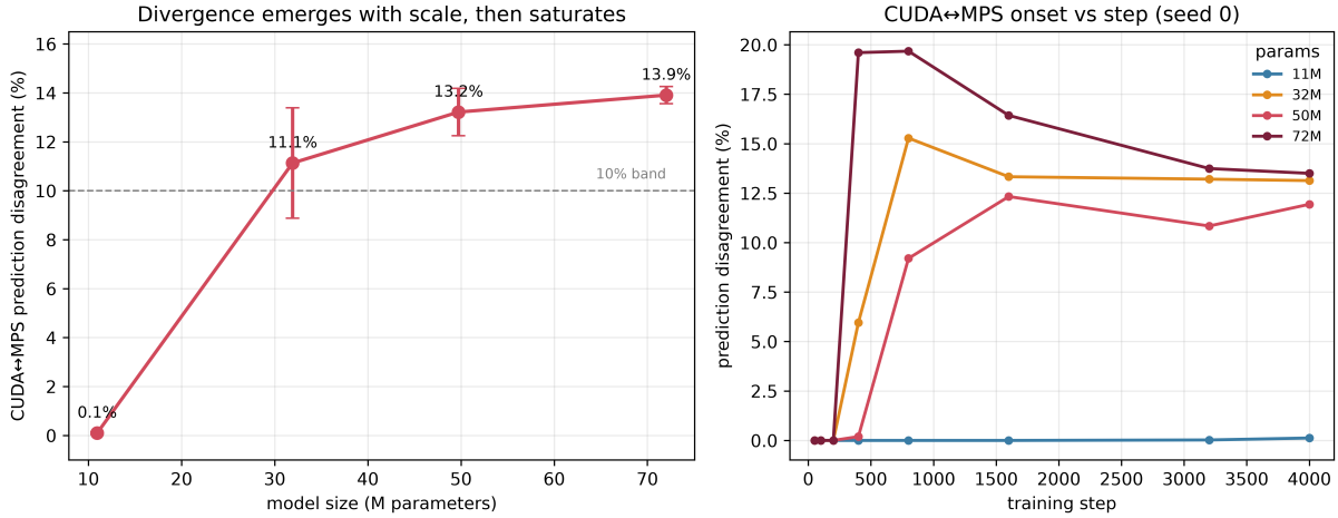
Figure 2: Cross-system (CUDA↔MPS) prediction disagreement and model scale. Left : final-step disagreement vs. model size (10.9M/31.9M/49.7M/72.0M parameters); markers are the mean over seeds {0, 1, 2}, error bars \pm 1 SD, dashed line the pre-registered 10% band. Divergence emerges sharply between 10M and 30M, then saturates. Right : disagreement vs. training step (seed 0) for the four sizes; the 11M model stays flat throughout training while the larger models cross onset by step 400–800.
