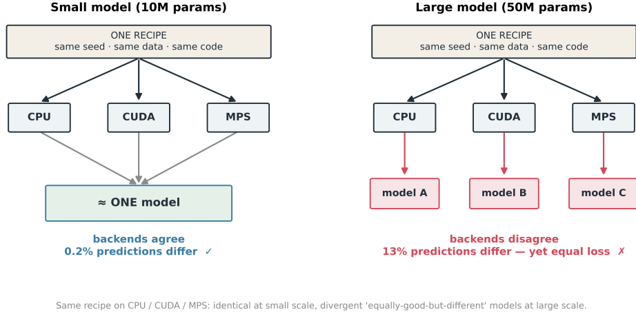
Figure 1: Graphical abstract. One training recipe (same seed, data, code) on CPU/CUDA/MPS yields a near-identical model at 10M (0.2% prediction disagreement) but divergent “equally-good-but-different” models at 50M (13.2%, equal loss).
