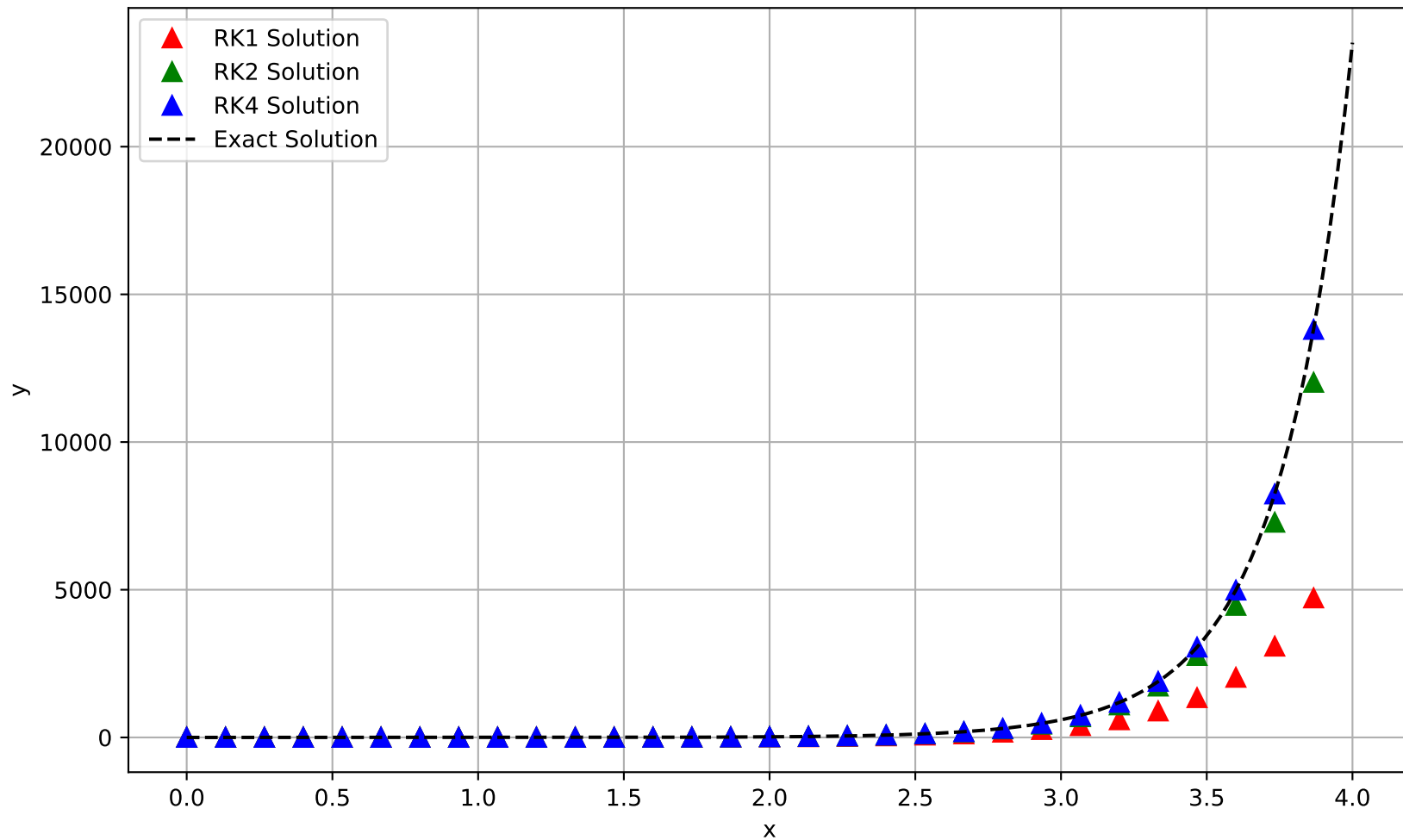
RK4 demo
