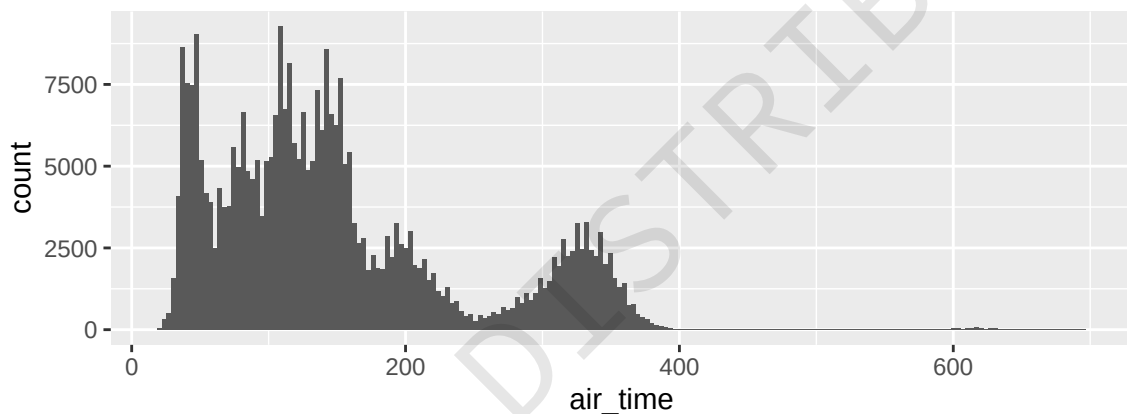
200 bins – too many peaks
