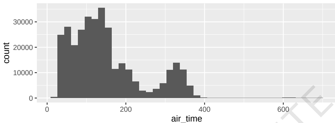
40 bins – reasonable detail
