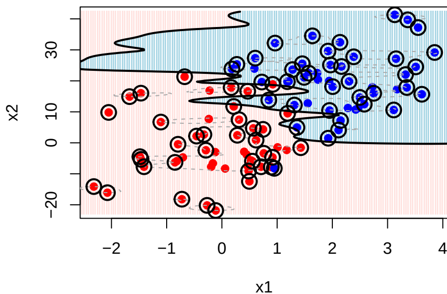
Radial kernel, unscaled predictors
