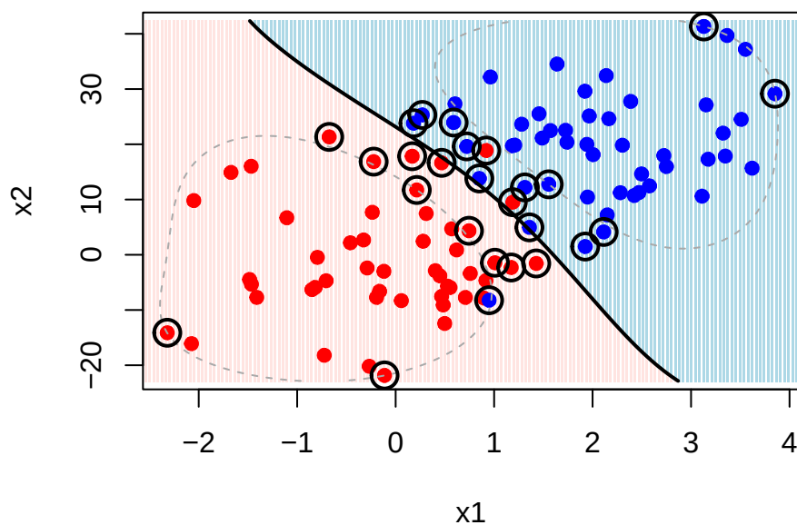
Radial kernel, scaled predictors
