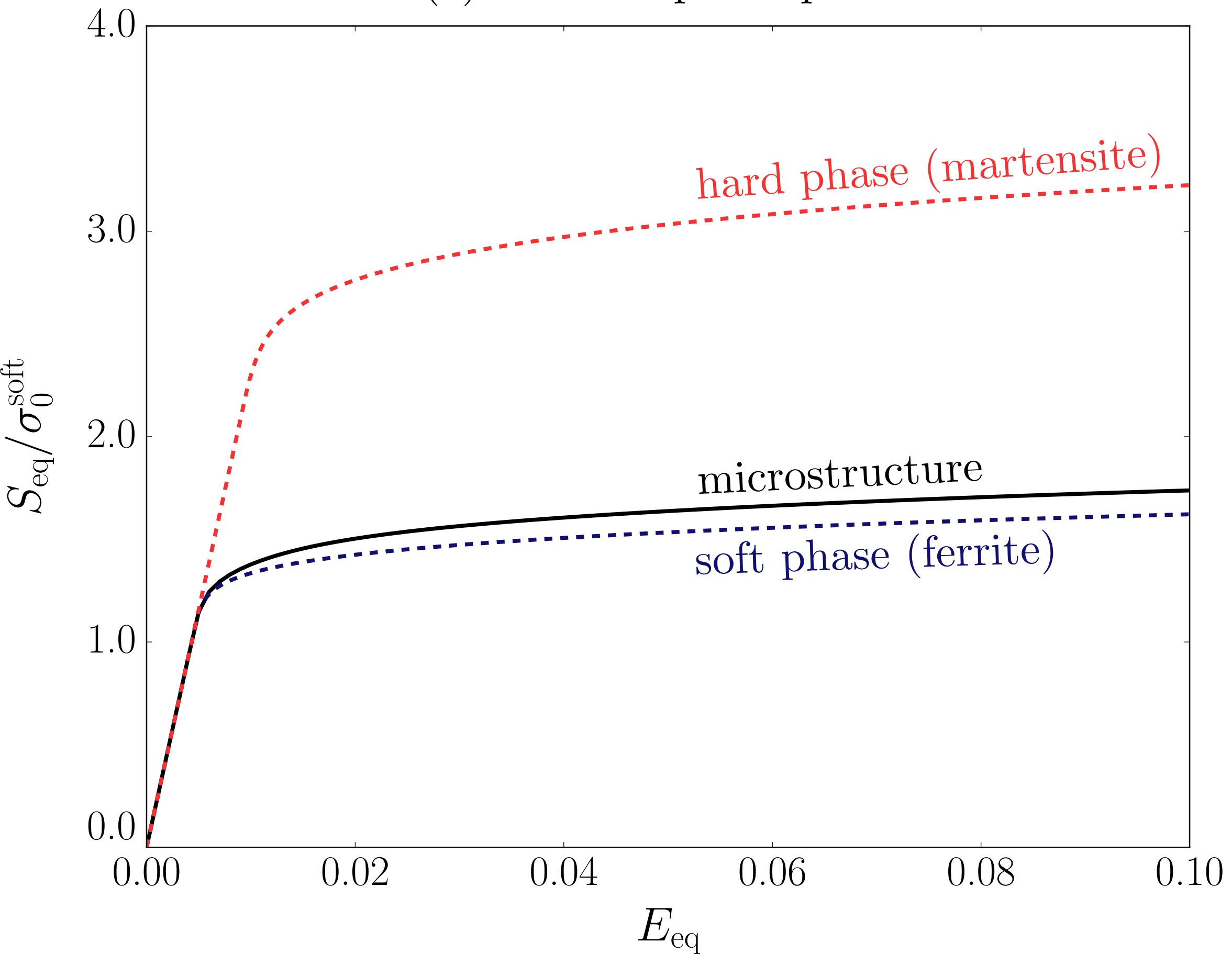
(a) macroscopic response
