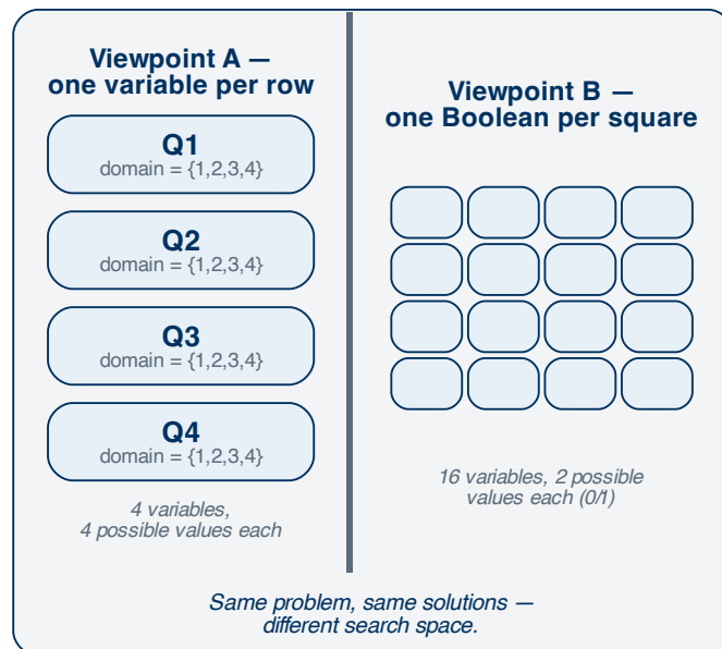
Figure 1.2: Two competing viewpoints for the same 4-queens instance.
