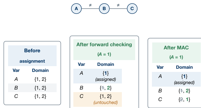
Forward checking versus MAC: domain updates after A = 1
