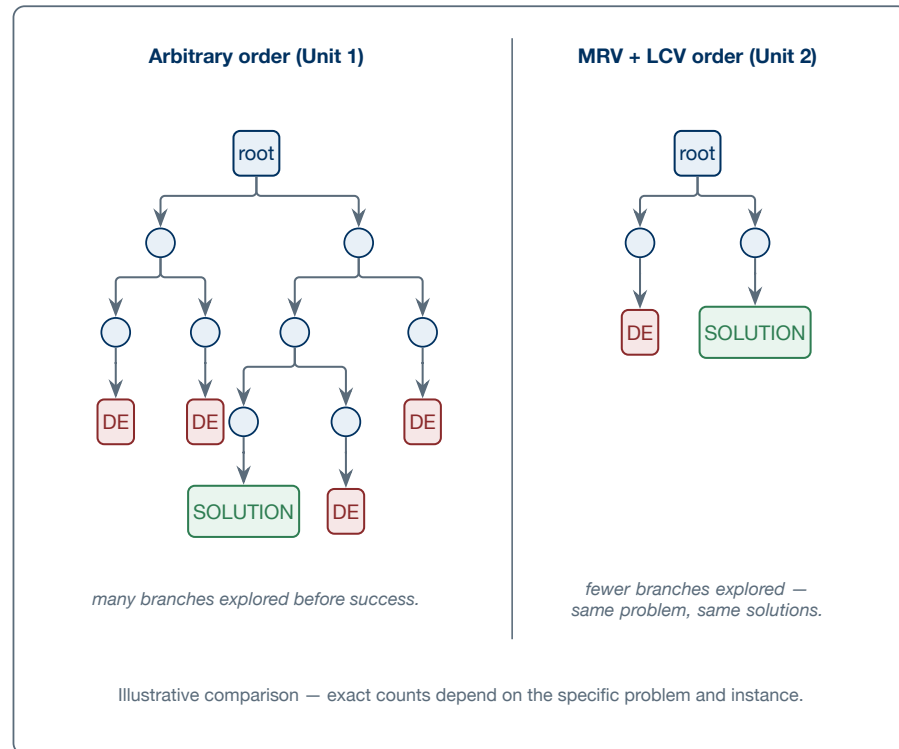
Figure 3.2: Schematic comparison of the same CSP explored under an arbitrary order (left) and under MRV plus LCV (right) – same problem, same solutions, a visibly smaller explored tree on the right.
