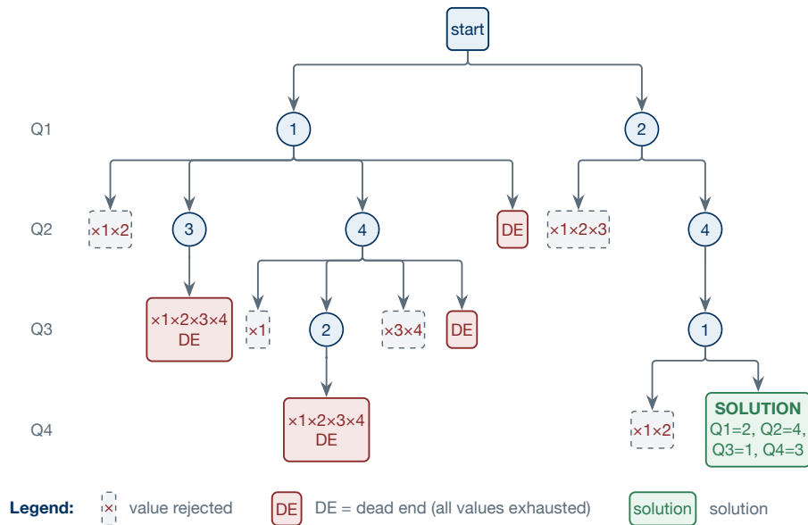
Figure 3.1: The full backtracking search tree for 4-queens under variable order Q_1, Q_2, Q_3, Q_4 and ascending value order – three dead ends under Q_1 = 1 , the solution Q_1 = 2, Q_2 = 4, Q_3 = 1, Q_4 = 3 under Q_1 = 2 .
