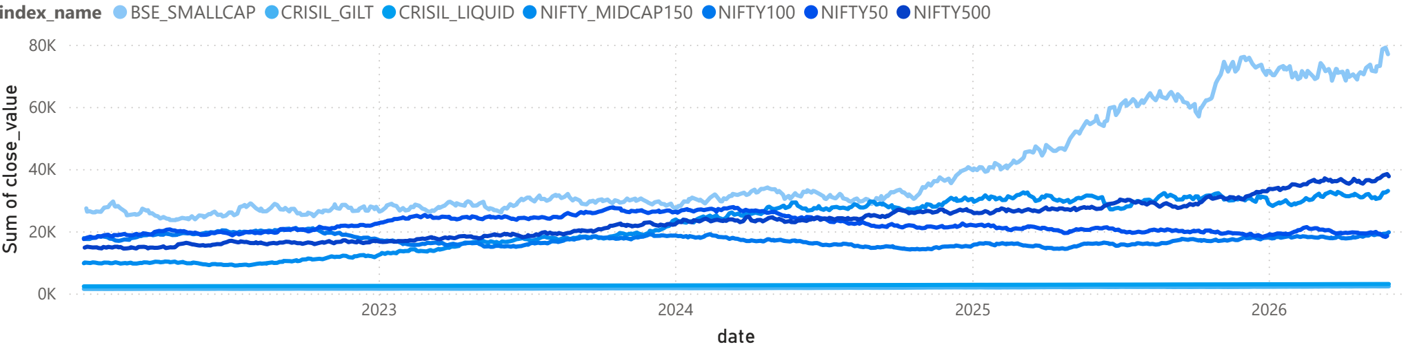
Benchmark Performance
