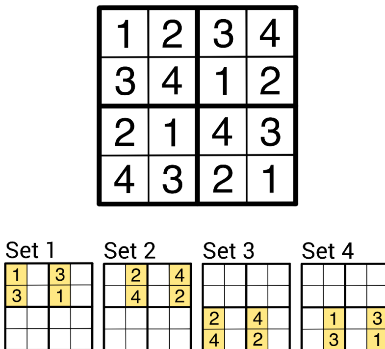
Figure 11: 4 unavoidable sets on a type-1 Shidoku board.
