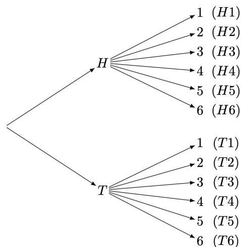
Figure 1: Tree diagram for Example 3, flipping a coin then rolling a die.
