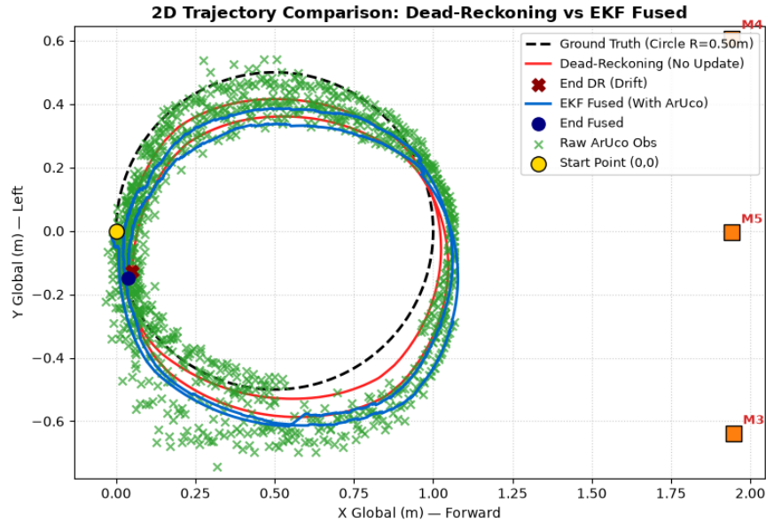
Figure 5.5: Circle trajectory compare
