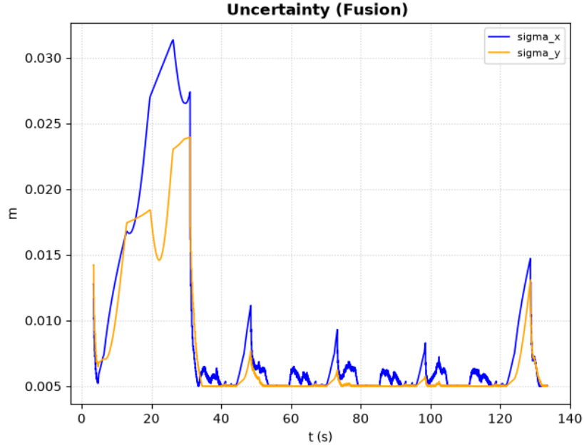
Figure 5.4: Uncertainty square EKF fusion trajectory
