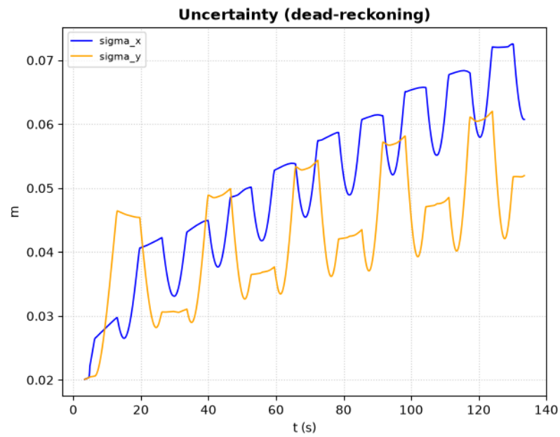
Figure 5.3: Uncertainty square dead reckoning trajectory
