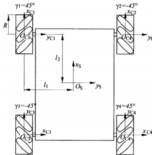
Figure 2.1: Mecanum kinematic
