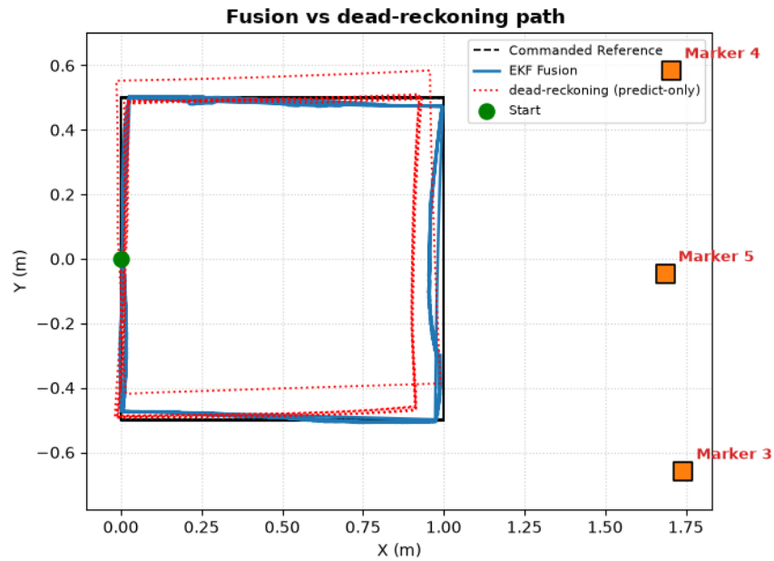
Figure 5.2: Square trajectory compare
