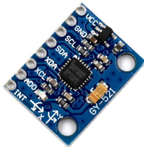
Figure 3.4: MPU-6050
