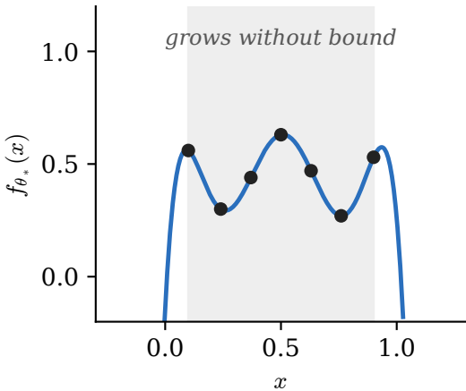
polynomial (degree 6)
