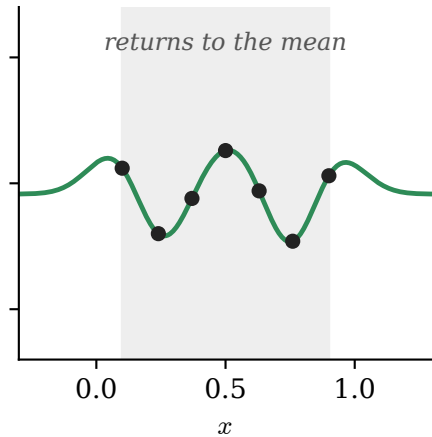
Gaussian bumps at the data
