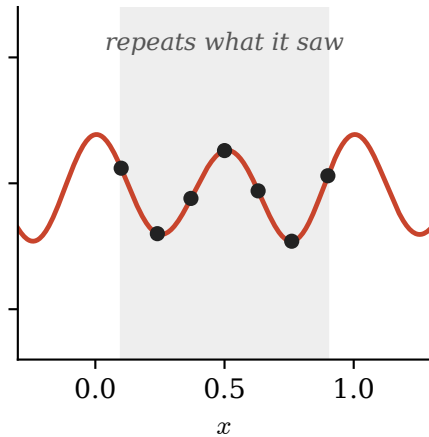
trigonometric (3 harmonics)
