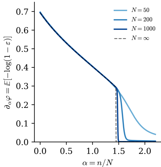
first derivative: sigmoid \rightarrow step
