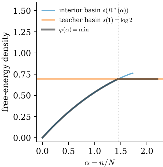
two basins cross at \alpha_c \approx 1.45
