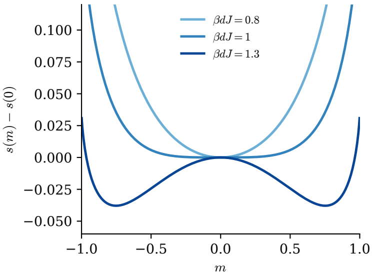
B = 0 : one basin splits in two at \beta_c dJ = 1
