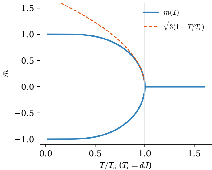
order parameter: continuous, kinked at T_c
