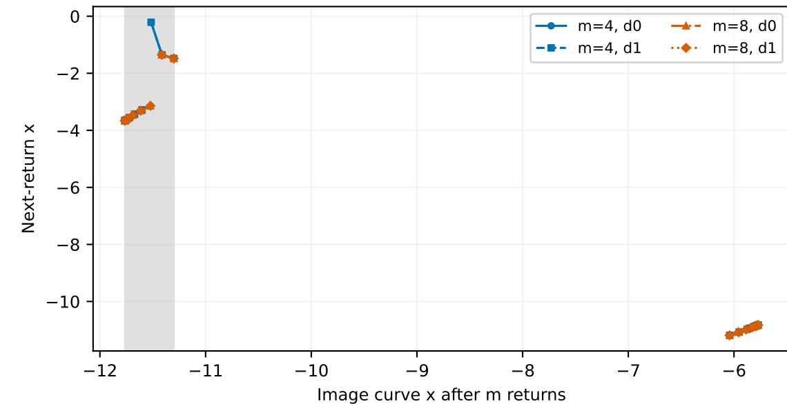
a=0.21575 , region 2: consistent
