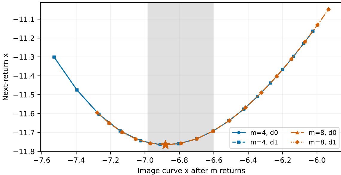
a=0.21577 , region 1: unresolved
