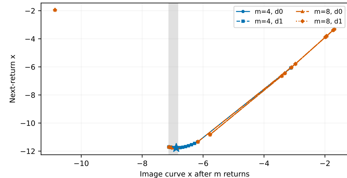
a=0.21577 , region 2: unresolved
