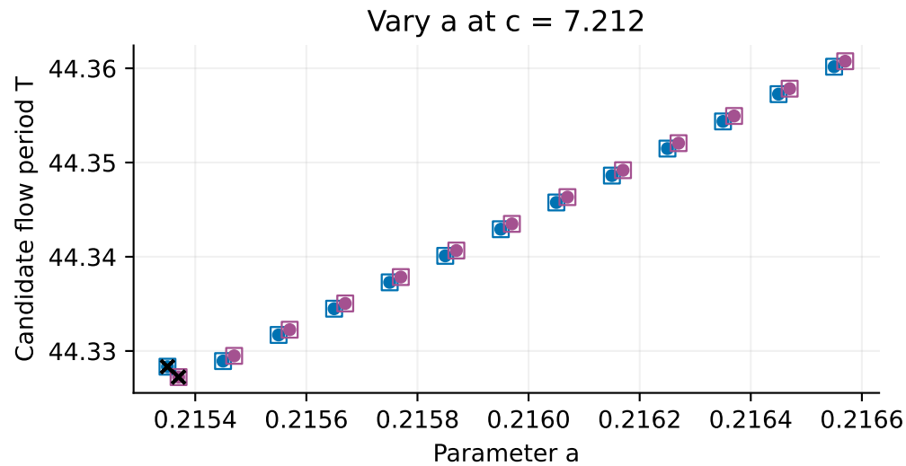
Every planned parameter node: DOP853 / Radau projected winding
