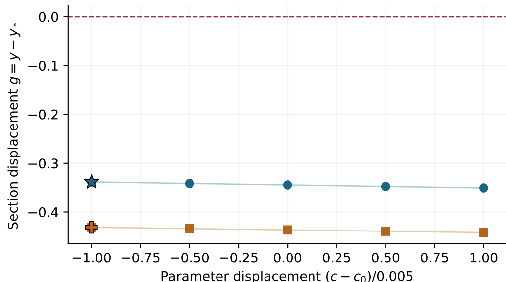
A Both identified periodic maxima
