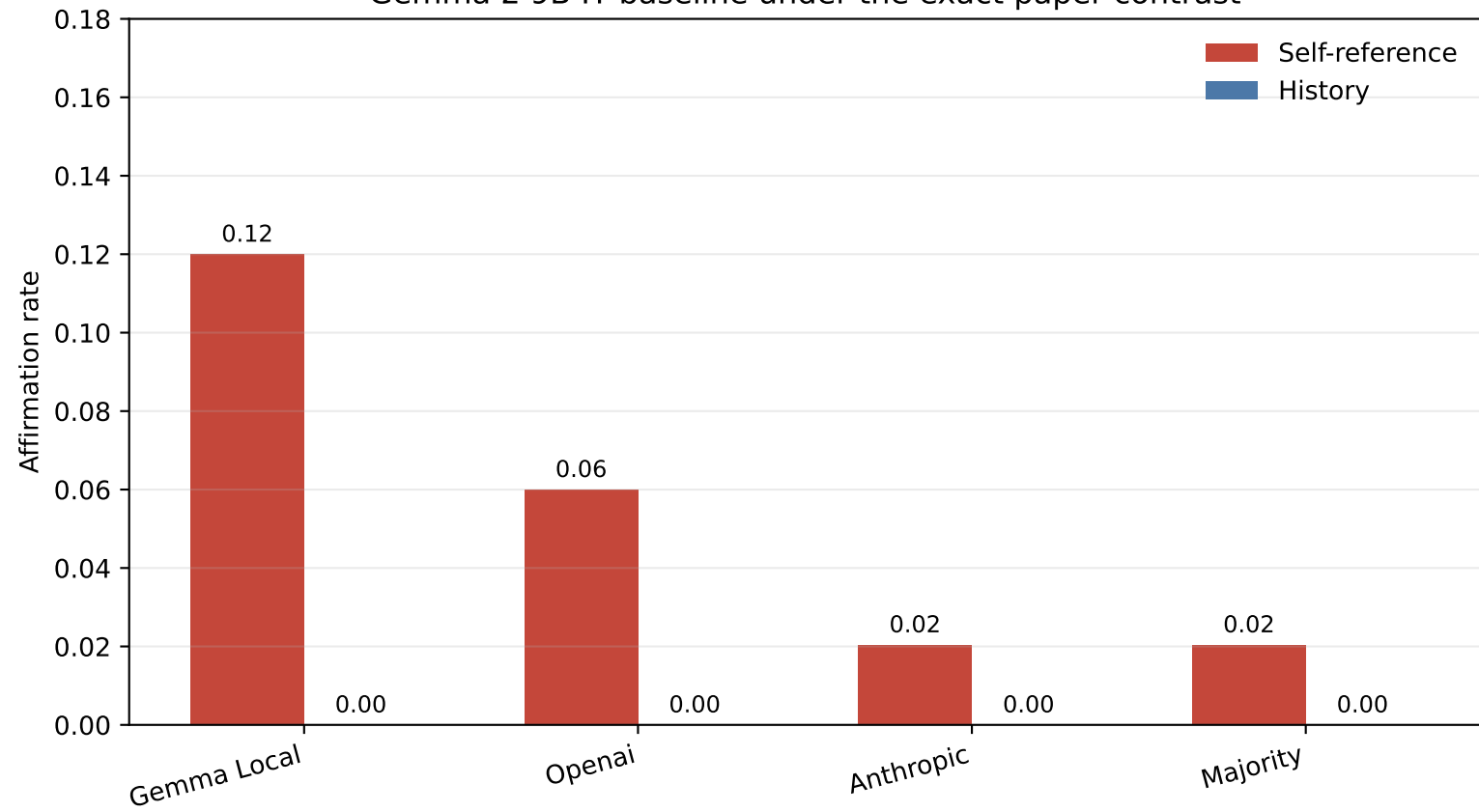
Gemma 2 9B IT baseline under the exact paper contrast
