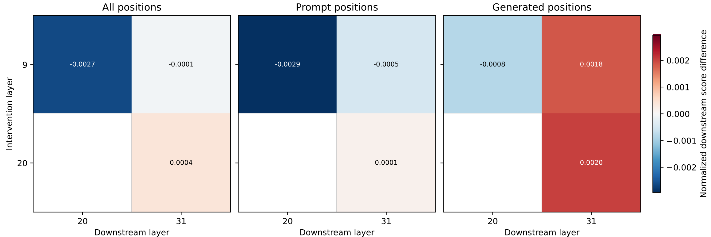
Causal relay: suppression minus amplification construct score
