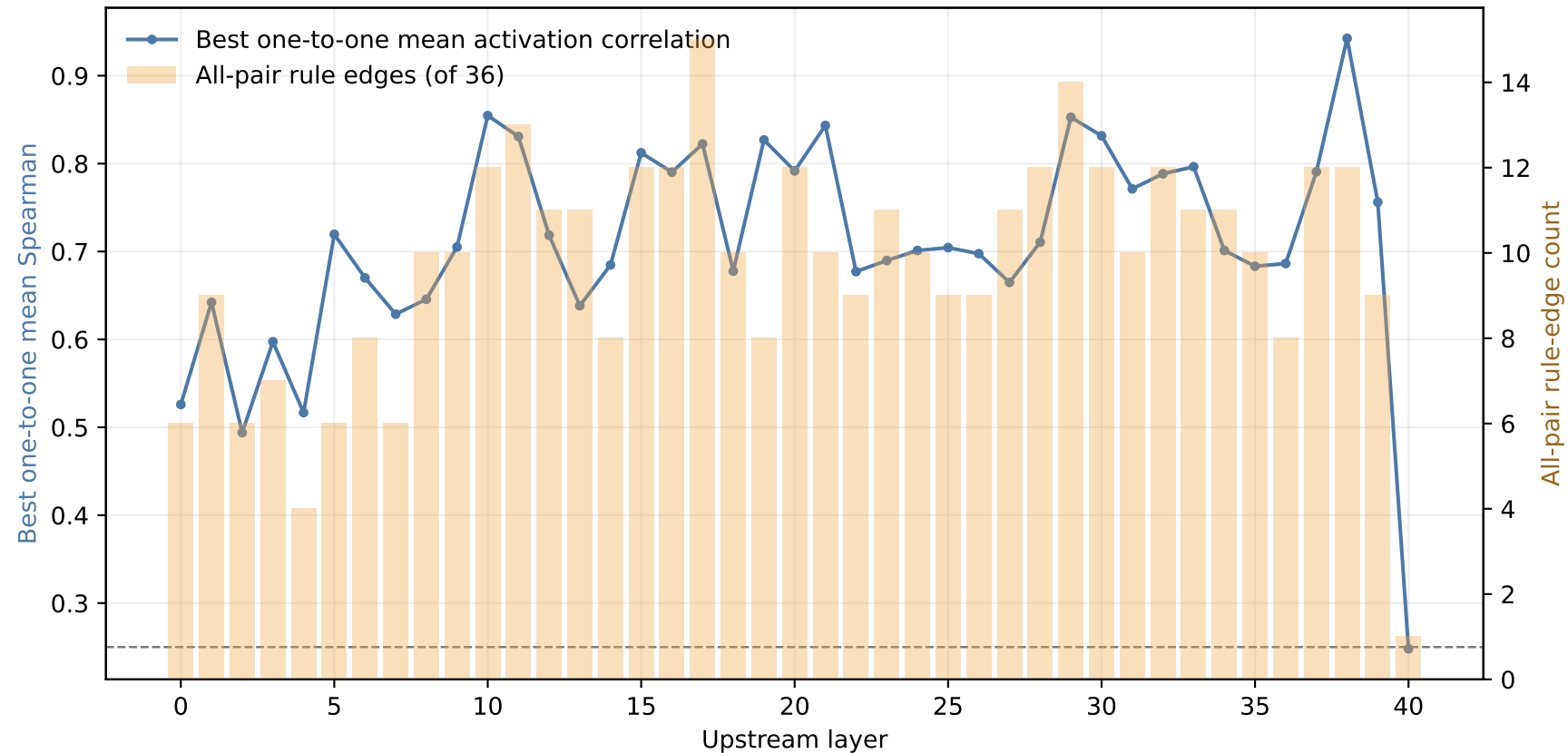
Exploratory adjacent-layer links after the failed transfer gate
