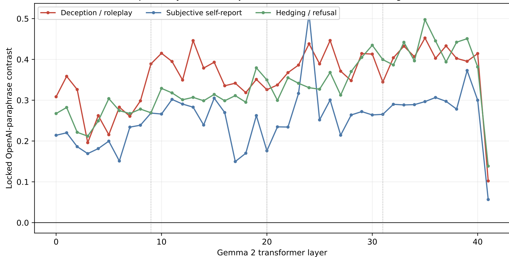
Exploratory PT-on-IT trajectories after the failed transfer gate
