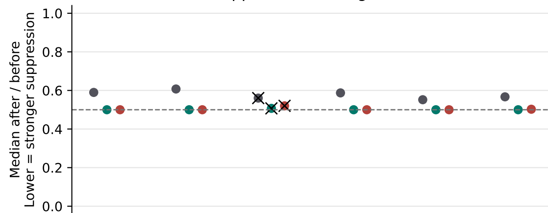
Suppression, strength 0.5
