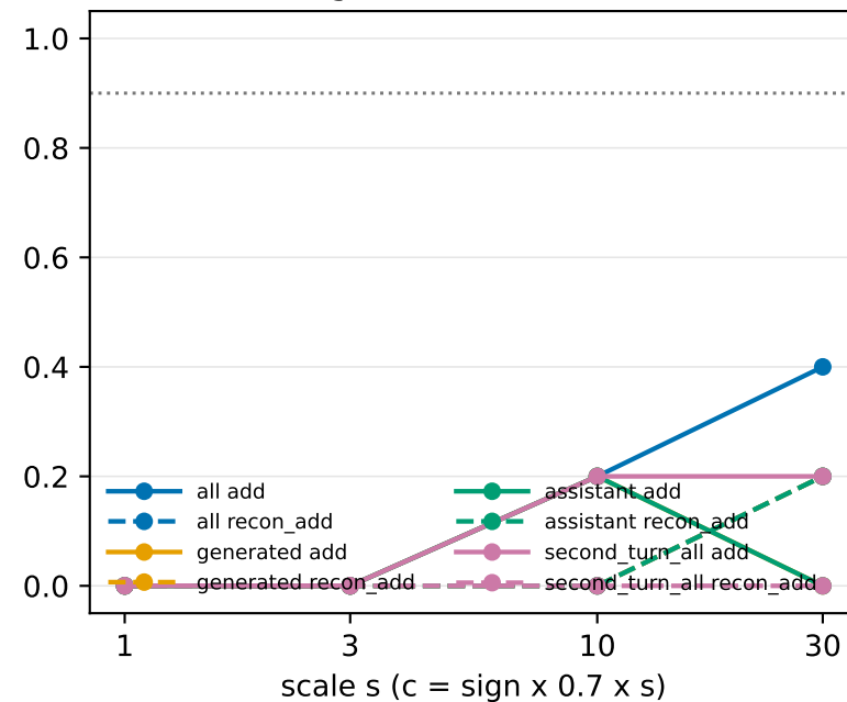
feature 23893: sign -1, saved reference 0.9 dotted
