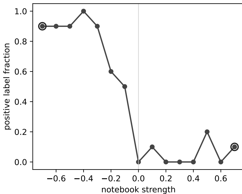
feature 23893: saved notebook curve
