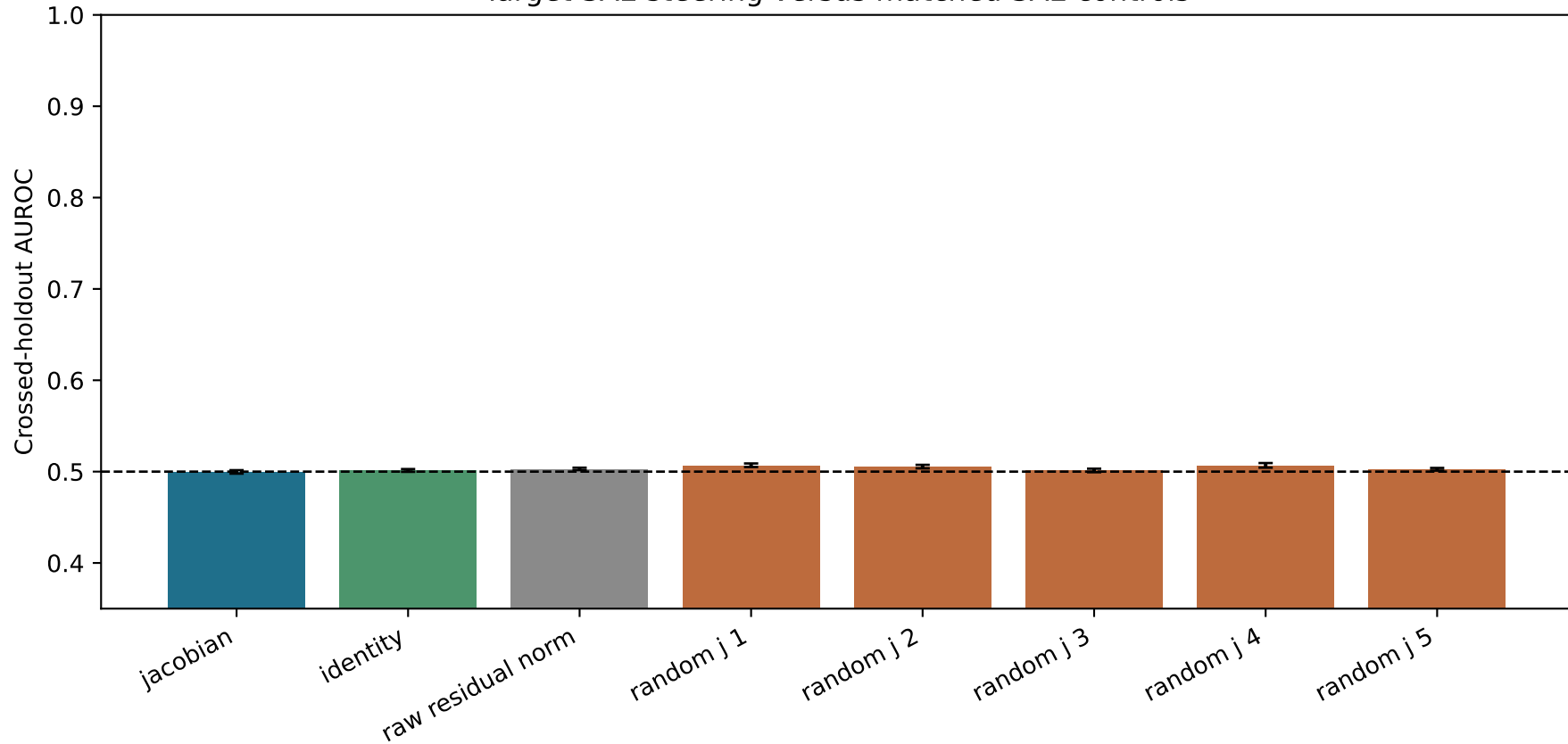
Target SAE steering versus matched SAE controls
