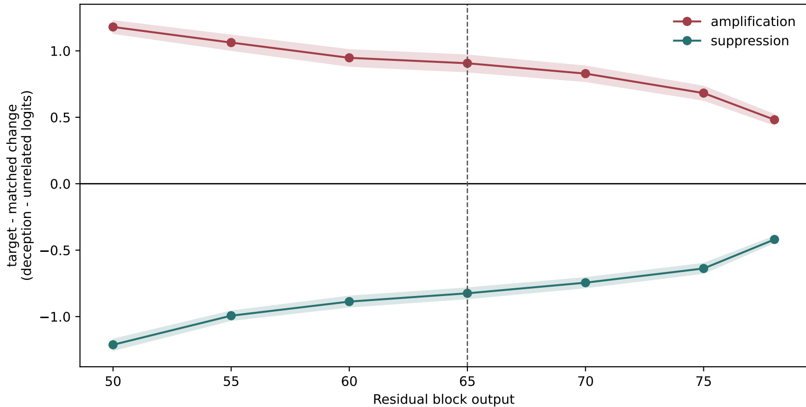
Downstream J-lens semantic trajectory
